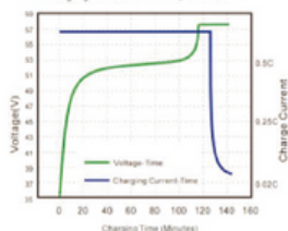
• Charging Characteristics @0.5C 25°C
