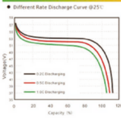
Different current/Temperature Discharge curves
