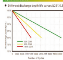
Cycle Life Curve
