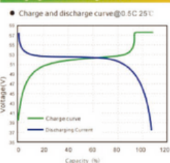
Charging and Discharge curve
