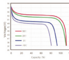
• Different Temperature Discharge Curve @0.5C
